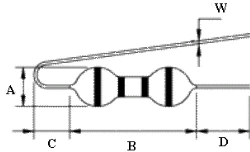
AL0307/0410/0510 TYPE
