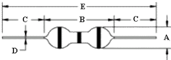
AL0204 TYPE
