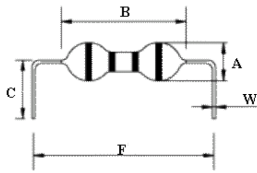
AL0307/0410/0510 TYPE
