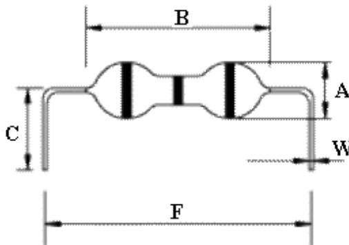
AL0204 TYPE
