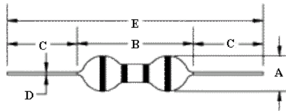
AL0307/0410/0510 TYPE
