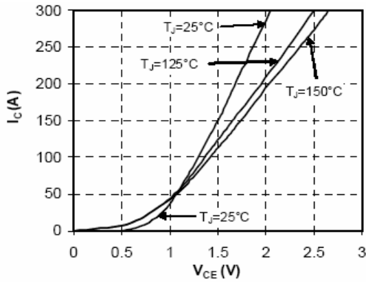
Fig 1. Typ. IGBT Output Characteristics
